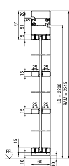
Vertical view single-leaf steel loft door
